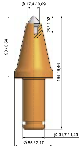
■ BSR255 BG32P-70.5590A Holder length 62 mm
