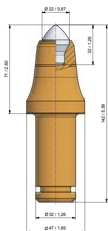
■ BSR332 BG32P-73.4771 Holder length 58 mm
