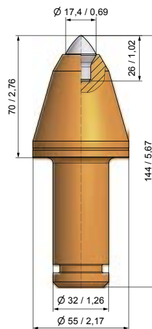
■ BSR269 BG32P-70.55.70C Holder length 61 mm
